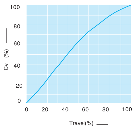
Linear characteristics
